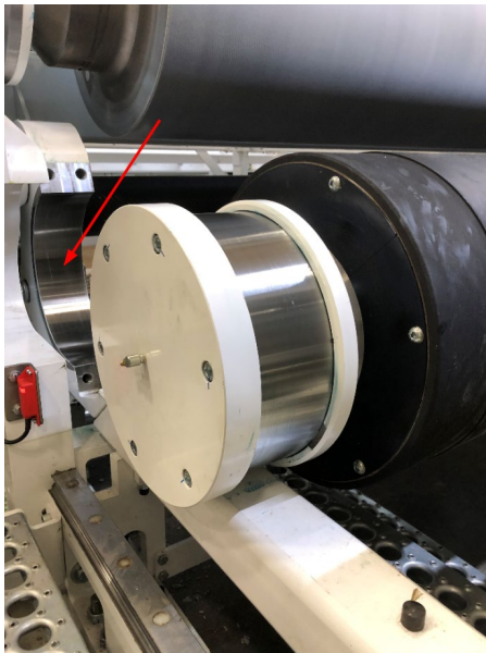
The Omnia's redesigned pivot arm decreases changeover time and reduces the risks inherent to overhead roll removal.
